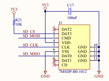
TF CARD
