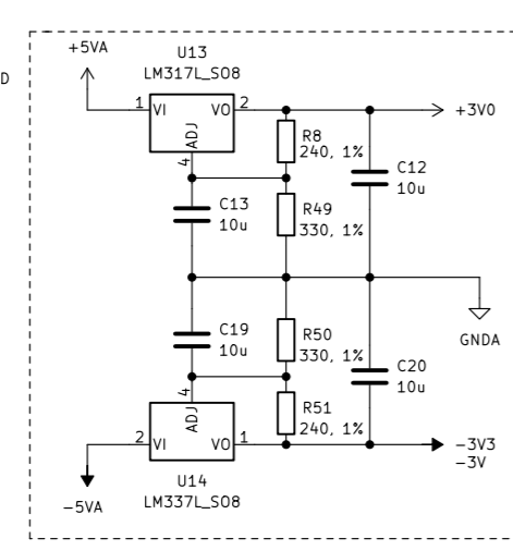
+ -3V for OPAMP circuit
