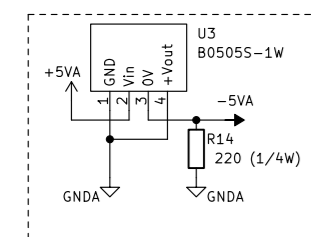
DCDC for -5VA
