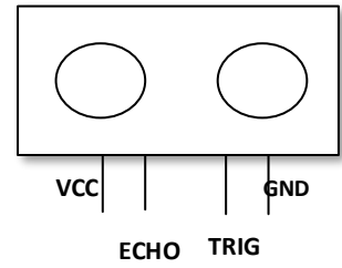
ULTRASONIC SENSOR
