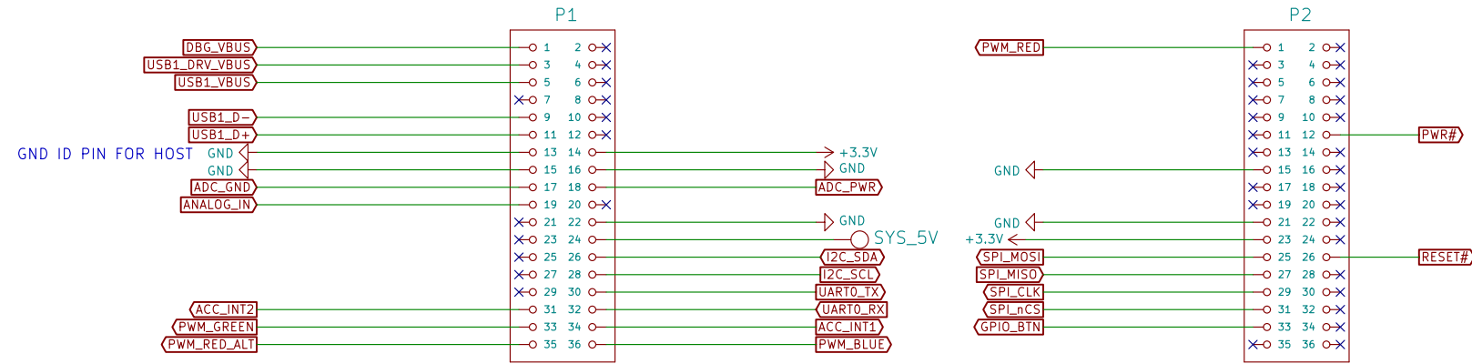
POCKETBEAGLE HEADERS
