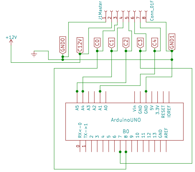
Arduino Uno I2C Master, Sensor Connections Layout
